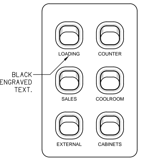
DETAIL C SP2 SWITCH PANEL NOT TO SCALE
