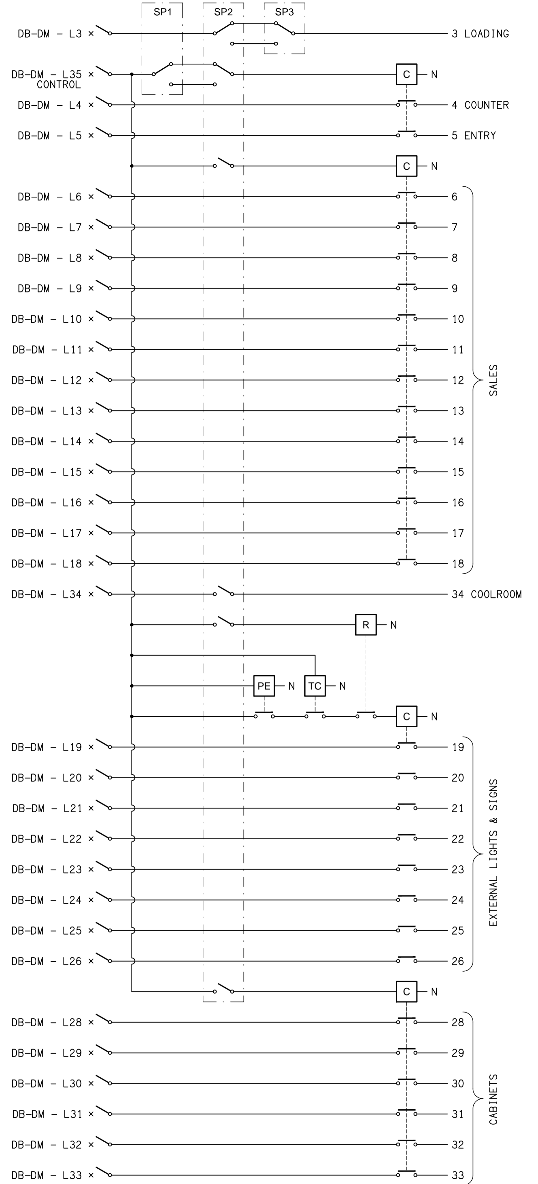
SCHEMATIC SP1, SP2, SP3 LIGHTING CONTROL NOT TO SCALE
