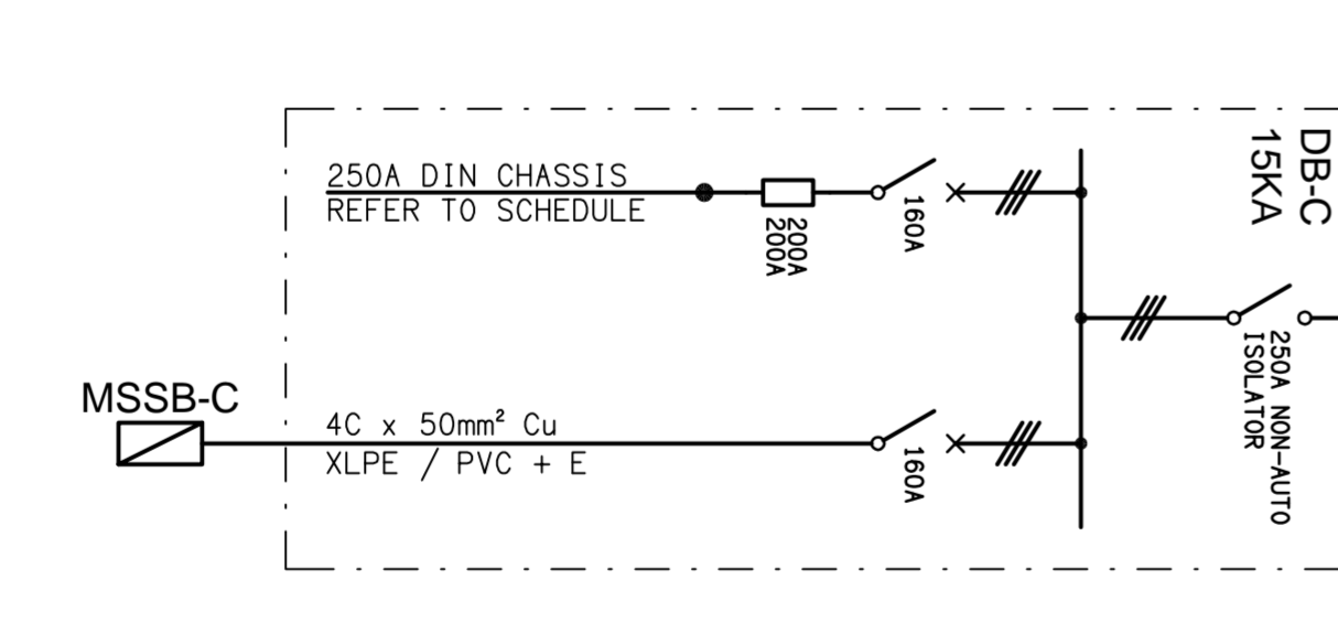
SCHEMATIC DISTRIBUTION BOARD DB-C NOT TO SCALE
