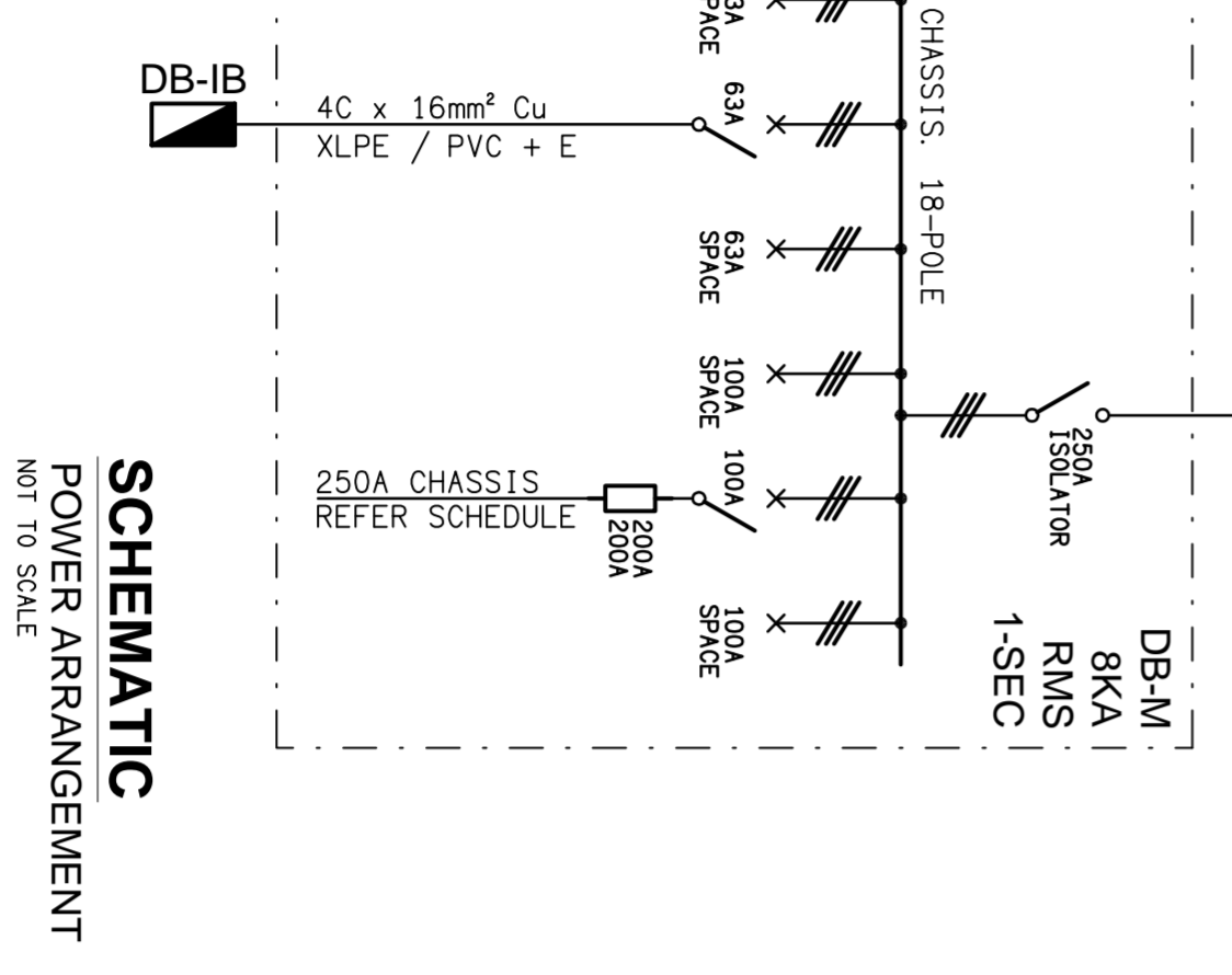
SCHEMATIC POWER ARRANGEMENT NOT TO SCALE
