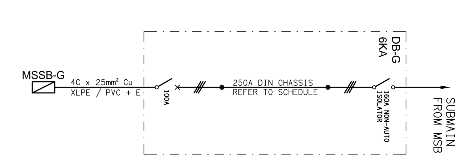
SCHEMATIC DISTRIBUTION BOARD DB-G NOT TO SCALE
