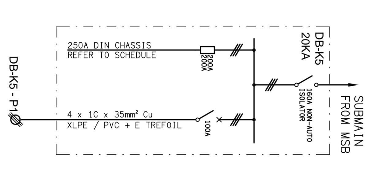
SCHEMATIC DISTRIBUTION BOARD DB-K5 NOT TO SCALE
