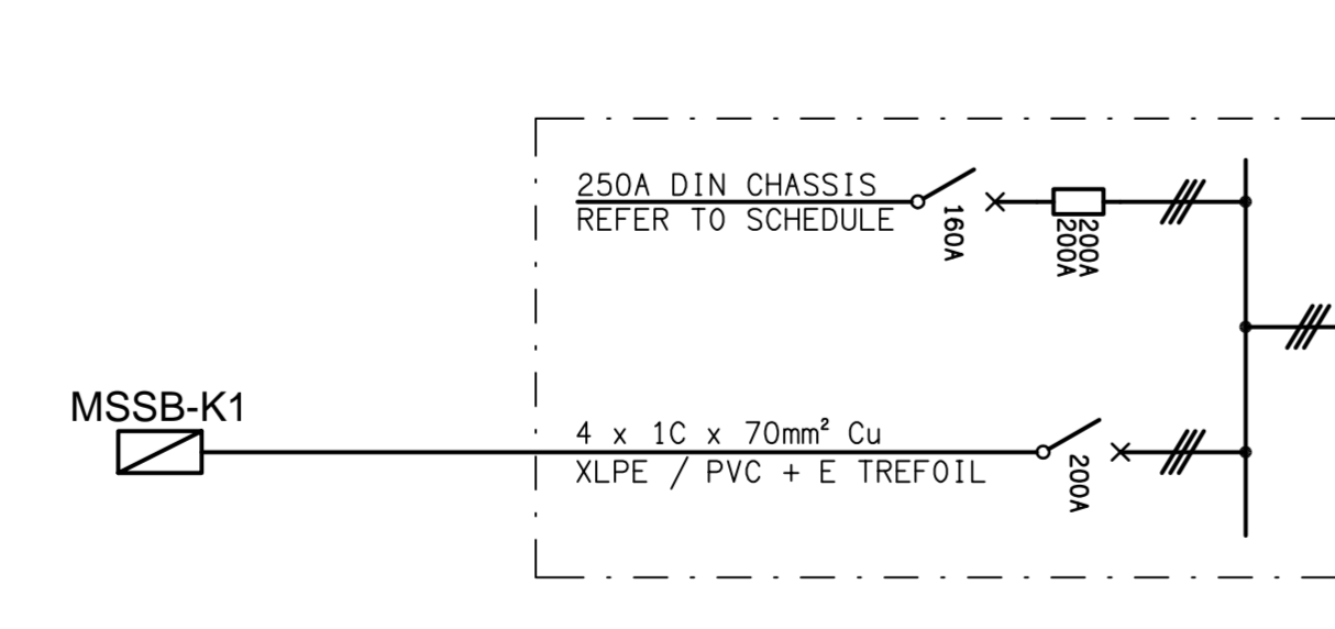
SCHEMATIC DISTRIBUTION BOARD DB-K1 NOT TO SCALE
