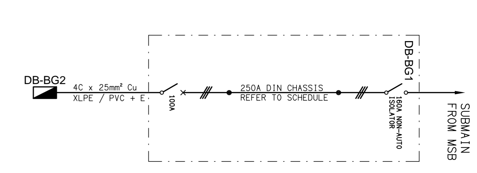
SCHEMATIC DISTRIBUTION BOARD DB-BG1 NOT TO SCALE
