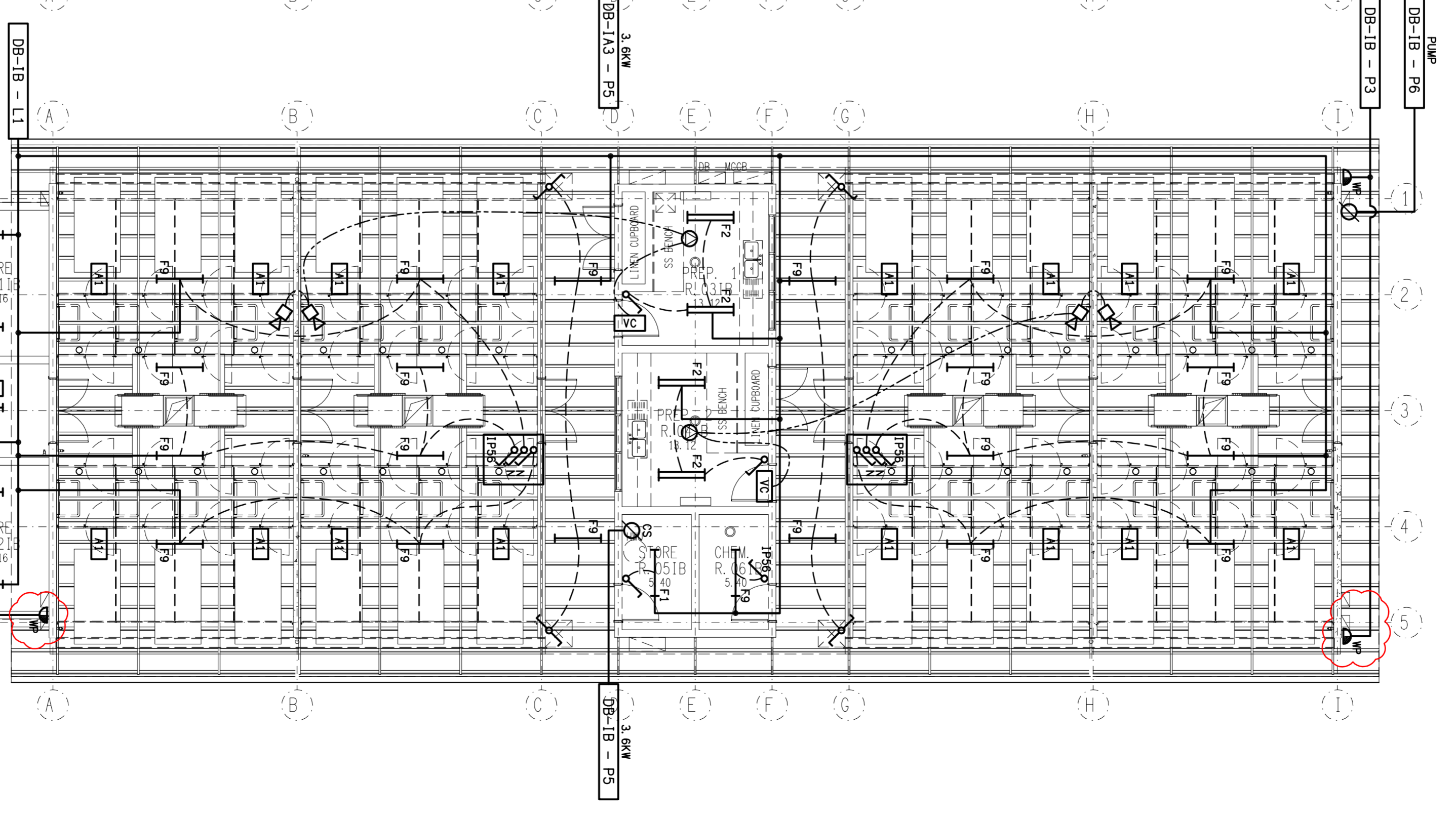
BUILDING IB PART FLOOR PLAN SCALE: 1:100
