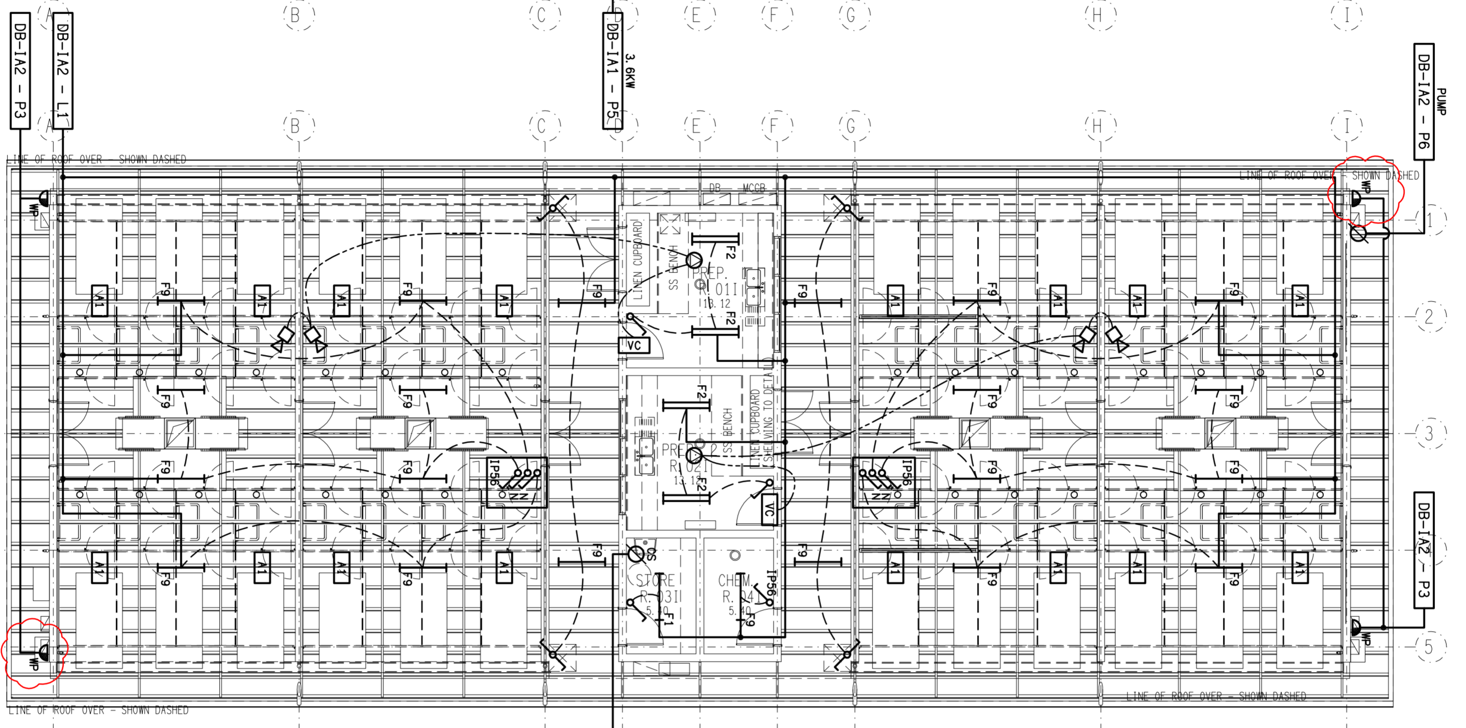
BUILDING IA BLOCK 2 PART FLOOR PLAN SCALE: 1:100
